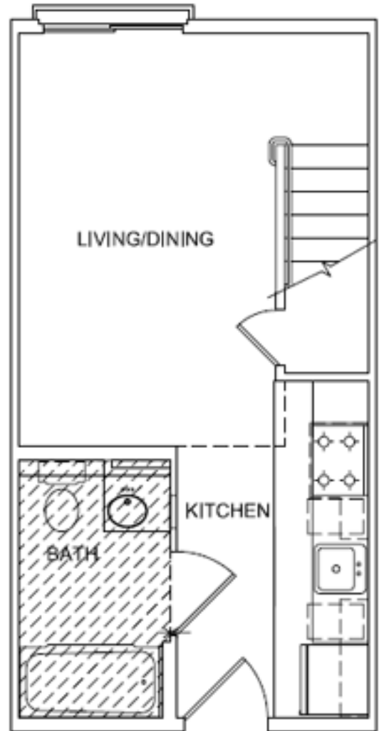
Studio With Loft (UNIT A.4)
